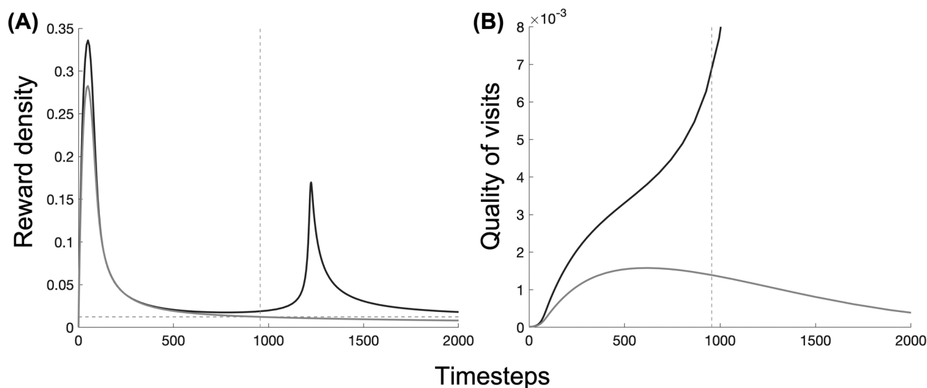
Figure 2. Reward threshold that determines invasion success during the transient dynamics. Transient dynamics are defined as the non-asymptotic dynamical regimes that persist for less than one to ‘as many as tens of generations’ (Hastings et al. 2018). Two simulations (one of the successful, black curves and one of the failed, gray curves, invasions) for the introduction of specialist plant species with high production of rewards and pollen attachability (Spec High R&P) chosen from the data shown in Fig. 1C, to illustrate: (A) an introduced plant species fails to invade (gray curve) when its rewards drop from the reward threshold (horizontal dashed line). The vertical dashed line indicates the timestep at which the reward threshold was crossed for the failed invasion. (B) The quality of visits received by the introduced plant species does not increase enough for the failed invasion before the reward threshold is reached, so it goes extinct (Supporting information). In the successful invasion, the introduced plant species is able to attract the pollinators’ foraging effort fast enough during the transient dynamics that it obtains enough quality of visits to persist before the threshold is met. The second peak observed in (A) corresponds to the increased floral rewards due to the increase in abundance of the introduced species that successfully invades, but then get depleted again to the reward density determining the system’s equilibrium (Supporting information). All successful and failed invasions look qualitatively the same as these figures.
